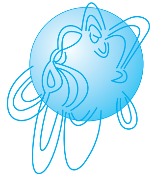
FIGURE 13-7 The field lines that describe the Sun's magnetic field structure at any given time are derived from ground-based measurements, for example, the Zeeman effect and the transport of charged matter. The high-intensity, chaotic structure is superimposed onto a constant general magnetic field of about 10^{-4} T.
